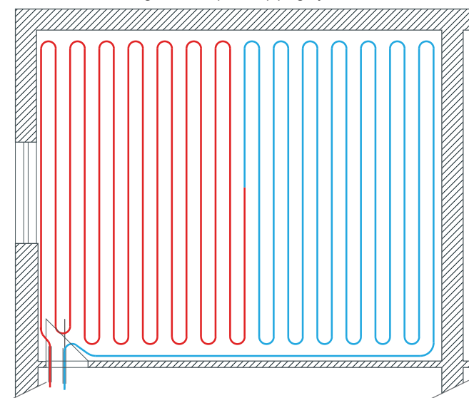
Figure 13: Serpentine piping layout
