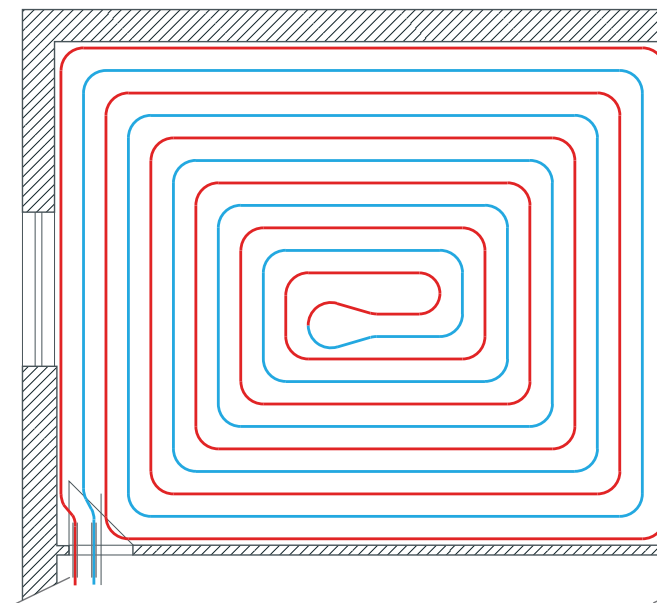
Figure 12: Counter flow piping layout
